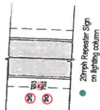
20mph Red Surface Entry Layout at junction (Antiskid textured surfacing)
