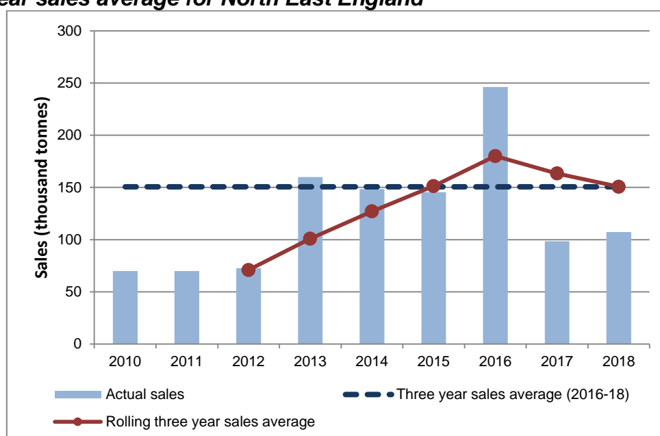
Figure 6.3: Comparison of actual sales of crushed rock imported by sea and the three year sales average for North East England
