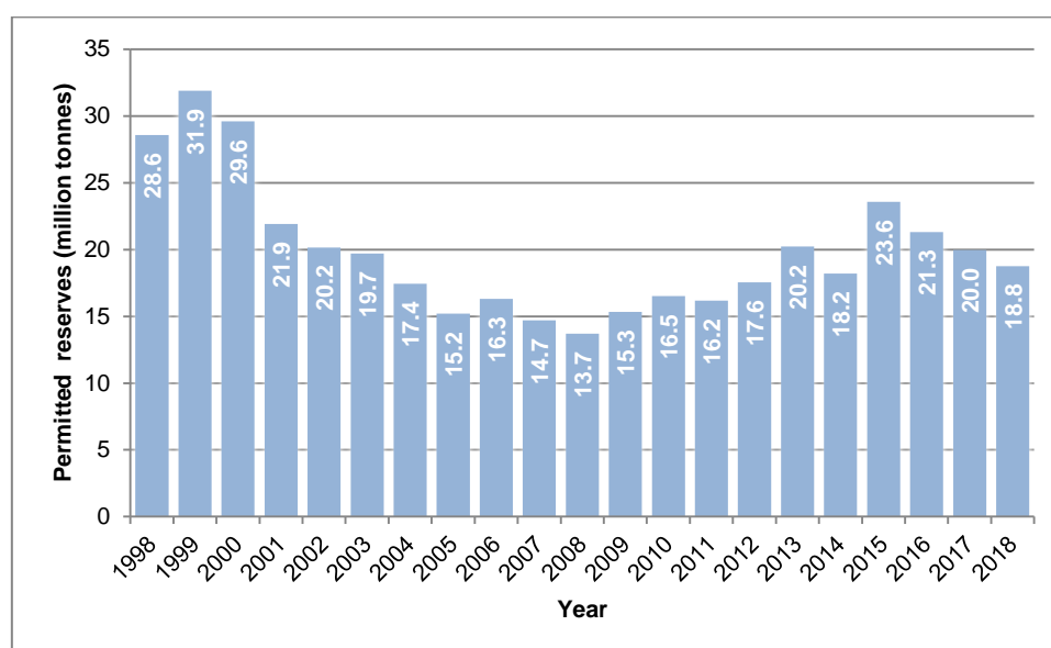
Figure 4.7: Comparison of permitted reserves of sand and gravel at quarries in North East England, 31 December 1998 to 31 December 2018
