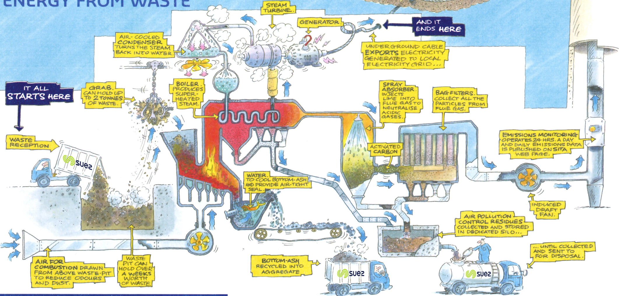
THE ENERGY FROM WASTE PROCESS
